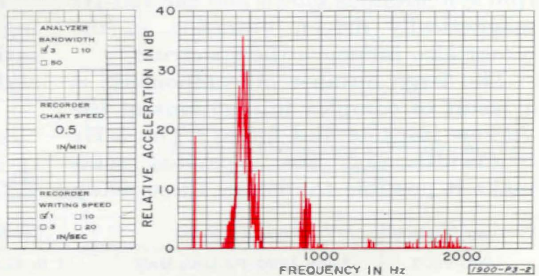
Figure 3. Analysis of the vibration of a frame holding a gear-belt drive. The frequency scale is sufficiently compressed to show the general character of the spectrum.
