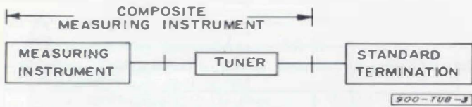
Figure 3. Standard termination attached to a composite measuring instrument.
