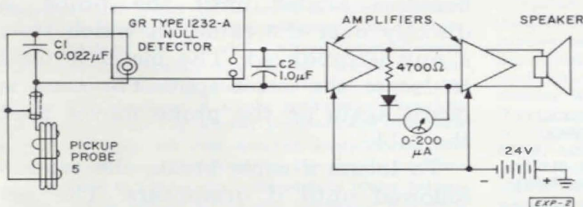
Figure 2. Elementary schematic of the receiving equipment.
