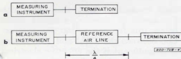
Figure 5. a) Setup to measure \Gamma_1 . b) Setup to measure \Gamma_2 .
