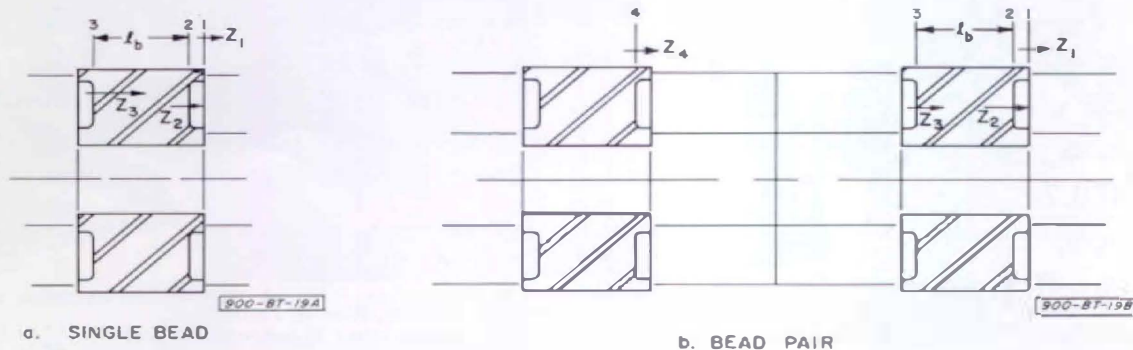
Figure 1. Cross-sections of GR900 dielectric support beads.
