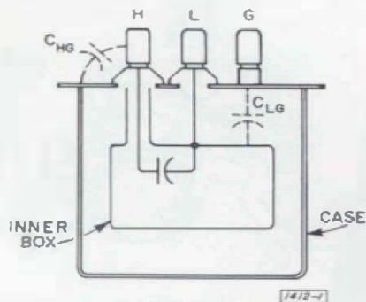
Figure 2. The double shielding used in the Type 1412-BC Decade Capacitor keeps C_{HG} very small. This capacitance is the difference between the three-terminal and two-terminal capacitance of the box; C_{LG} is approximately 125 pF.
