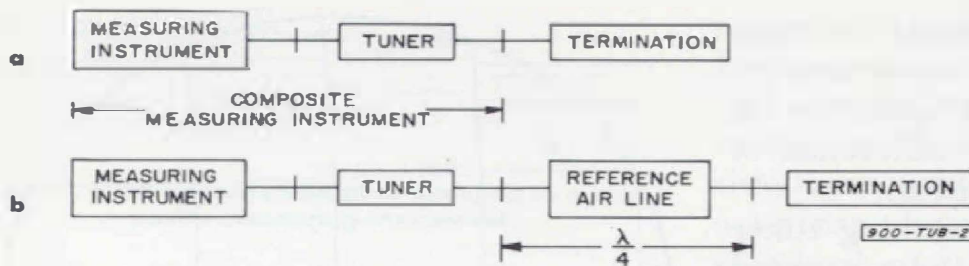
Figure 7. a) Setup to adjust \Gamma_1 to zero. b) Setup to measure \Gamma_2 and to determine \Gamma_1 directly.
