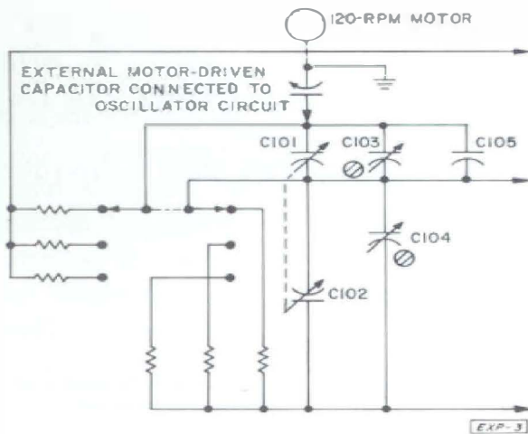
Figure 3. To produce a warble tone, a motor-driven capacitor is connected to the oscillator-tuned circuit.
