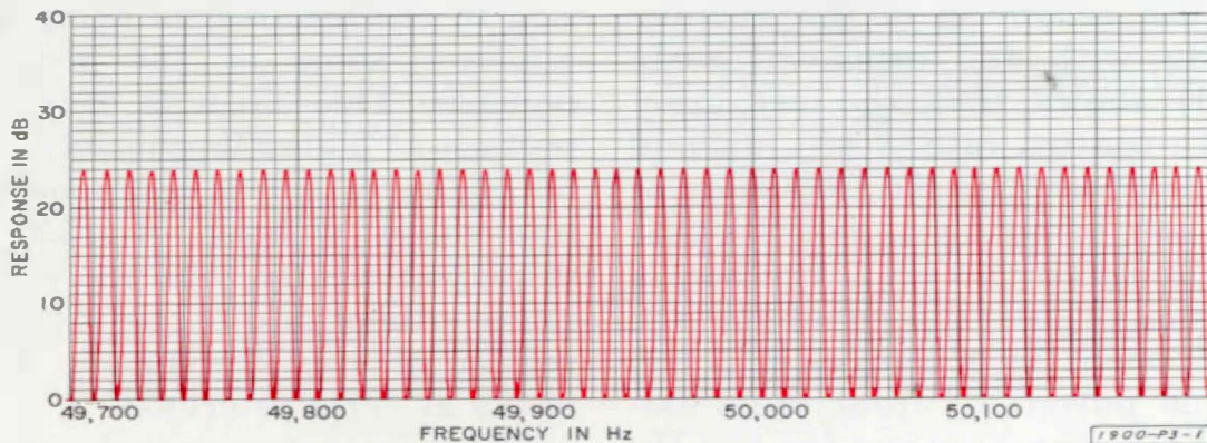
Figure 2. Section of a frequency spectrum in the vicinity of 50,000 Hz of a 30- \mu s pulse repeated every 0.1 s. The expanded frequency scale is used to show the individual components every 10 Hz.
