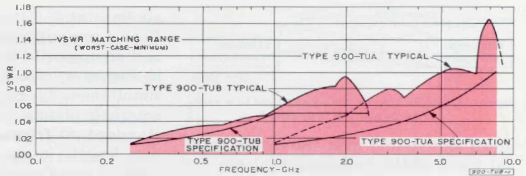
Figure 1. VSWR matching range of the Types 900-TUB and -TUA Tuners. Specifications and data shown are under the most restrictive phase conditions of the reflection to be matched out.
