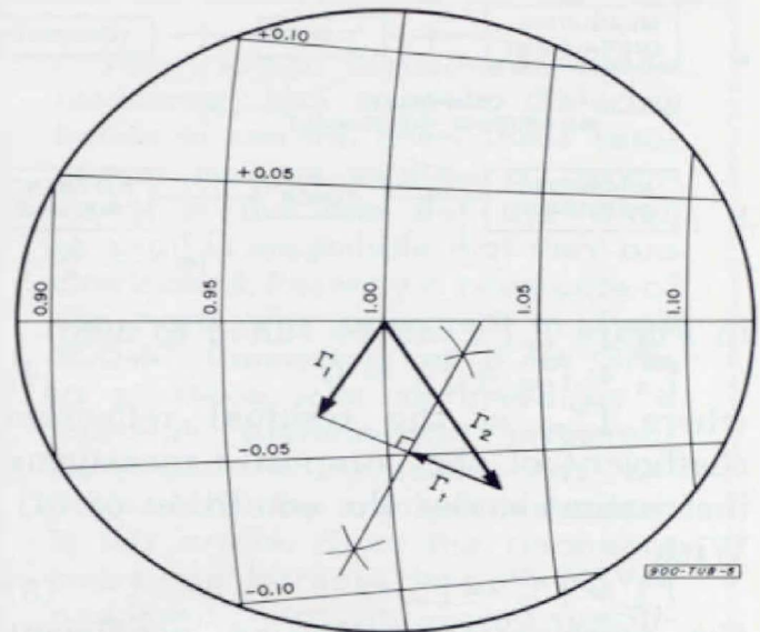
Figure 6. Smith Chart construction to determine \Gamma_t .
