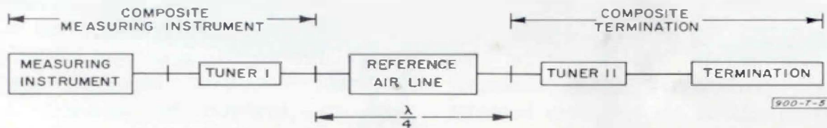
Figure 4. Setup for matching composite measuring instrument and composite termination to the characteristic impedance of an air-line standard.
