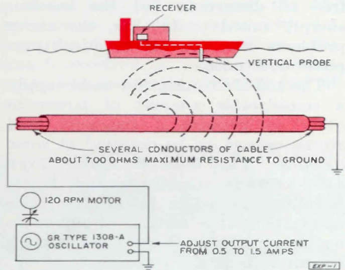
Figure 1. A signal is applied to the cable as shown, generating a magnetic field, which is detected by a probe and receiving equipment in the launch.
