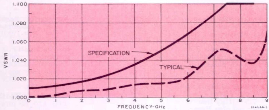
Figure 1. Type 874-LBB VSWR.
